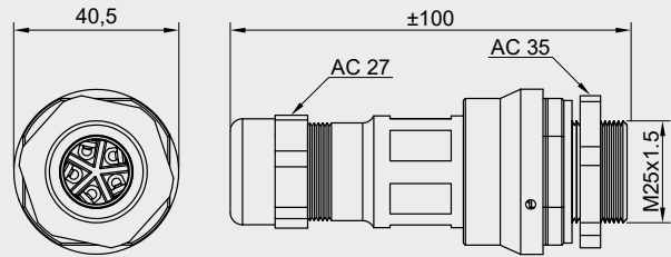
5-Pole connector
