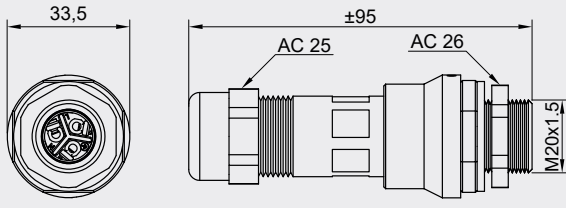
3-Pole connector
